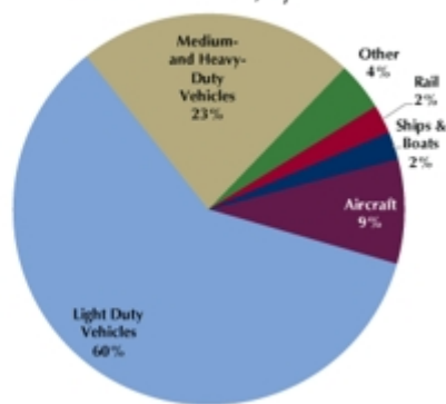
2013 U.S. Transportation Sector CO2 Emissions, by Source
