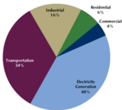
2013 U.S. CO2 Emissions, by Sector
